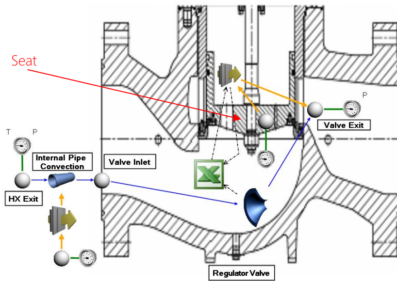
Figure 3: The Flownex® model used for analysis.
