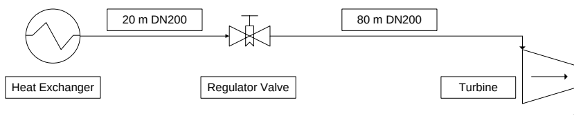
Figure 2: Flow path of the gas
