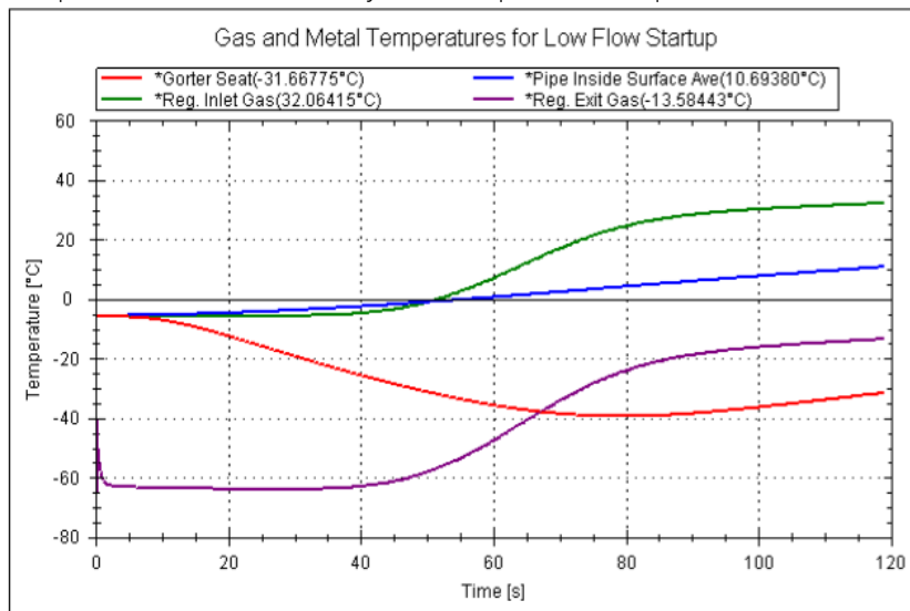
Figure 4: Flownex® temperature results of the gas and the valve seat.
