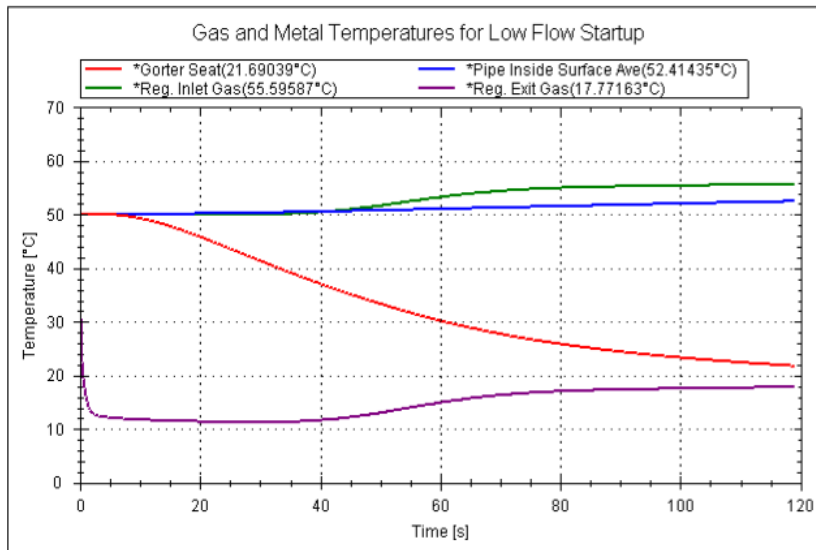
Figure 5: Flownex® temperature results of the gas and the valve seat (with trace heating).
