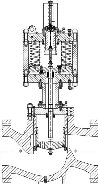
Figure 1: Cross section of a Pressure Regulating Valve.
