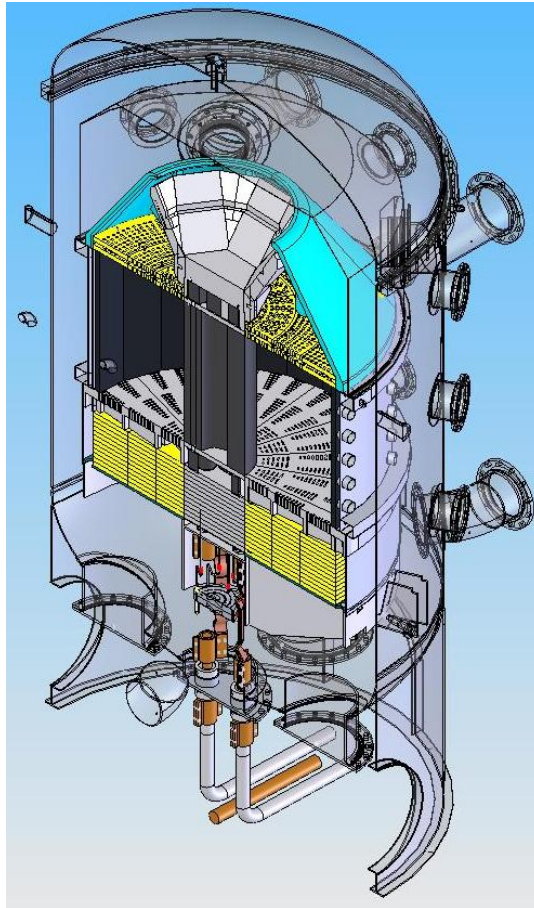
Figure 1: Section through the test section.
