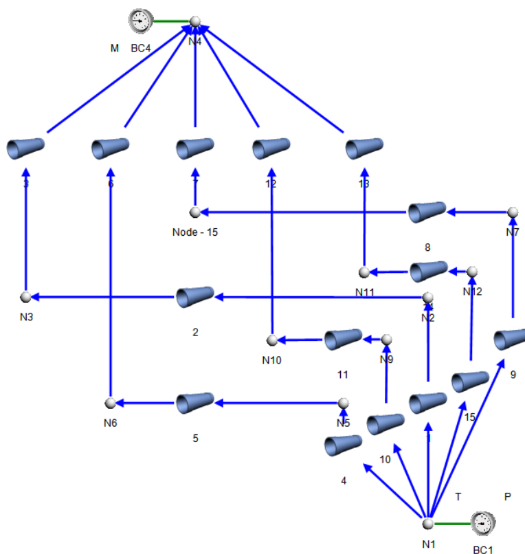
Figure 4: Flownex network of a single flow distribution manifold block.
