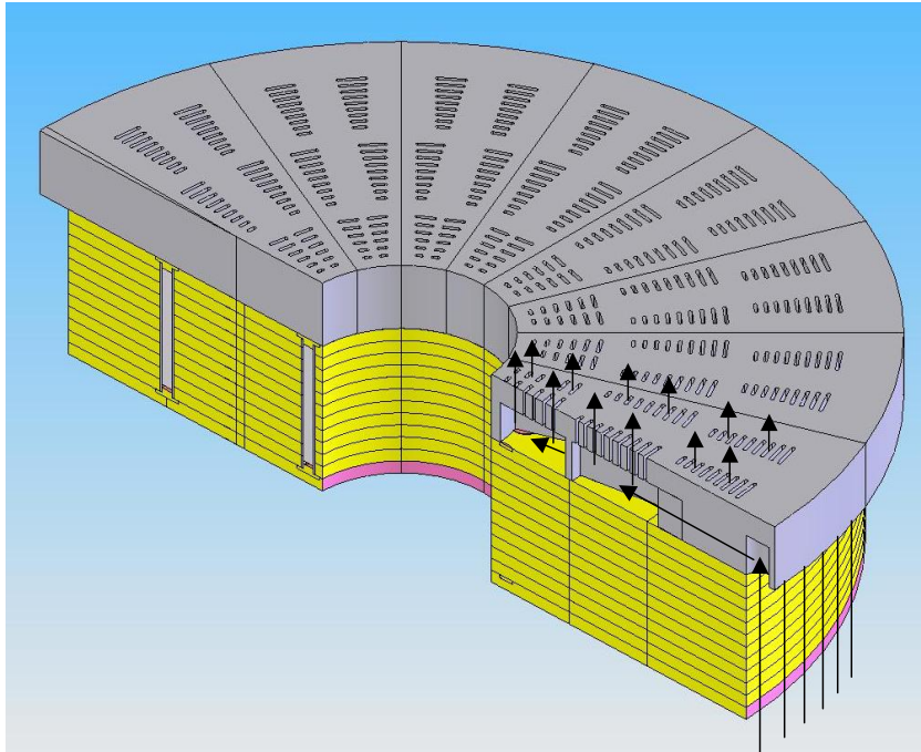
Figure 2: Section through the insulation layers and perforated flow distribution manifold.
