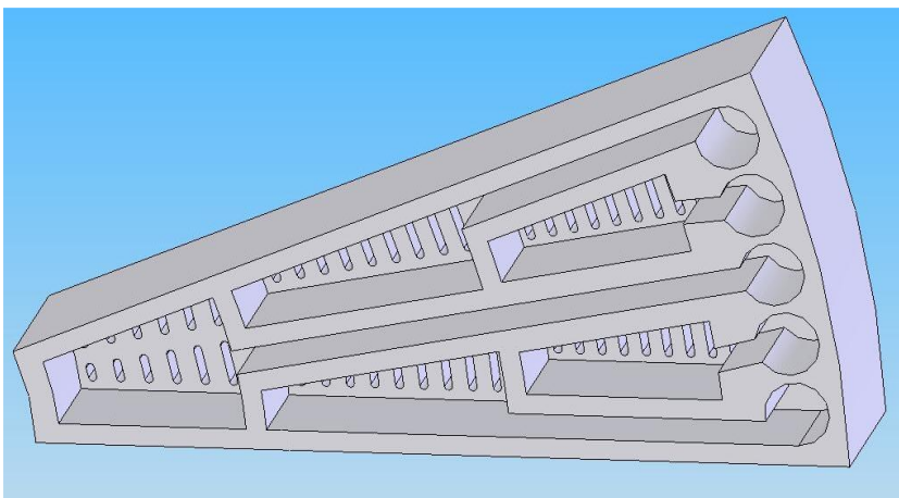
Figure 3: Detail of the perforated flow distribution manifold.
