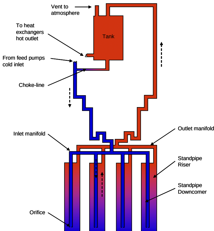
Figure 1: Schematic layout of one RCCS subsystem.
