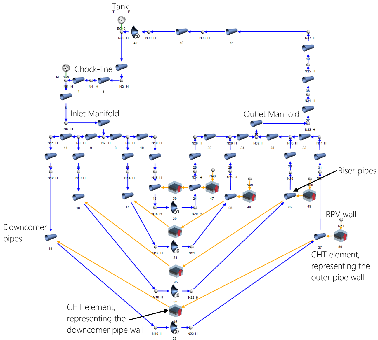
Figure 3: Flownex network of the RCCS with radiation from the RPV.
