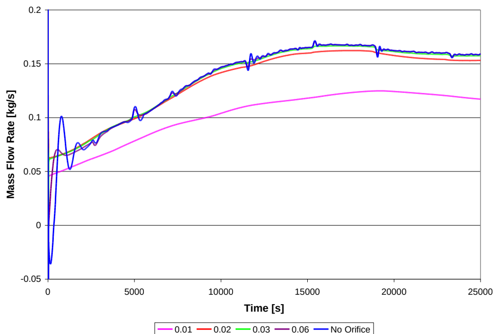
Figure 5: Passive mode: Standpipe mass flow rate for a 0.02 [m] choke-line.
