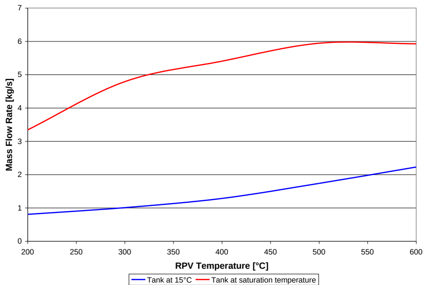
Figure 7: Total system mass flow rate vs. RPV temperature.
