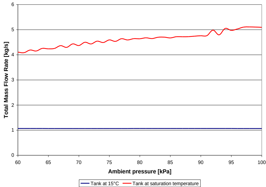
Figure 6: Total system mass flow rate vs. ambient pressure.
