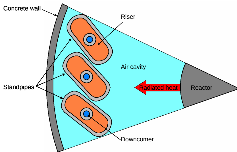
Figure 2: Top view cutout of the RCCS-Reactor configuration.
