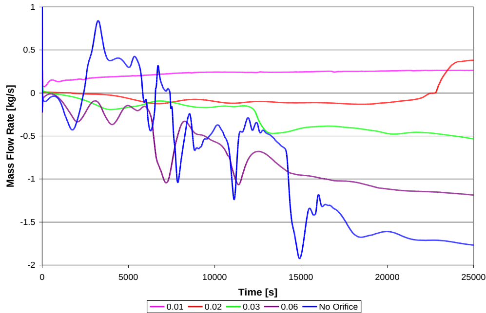
Figure 4: Passive mode: Standpipe mass flow rate for a 0.01 [m] choke-line.
