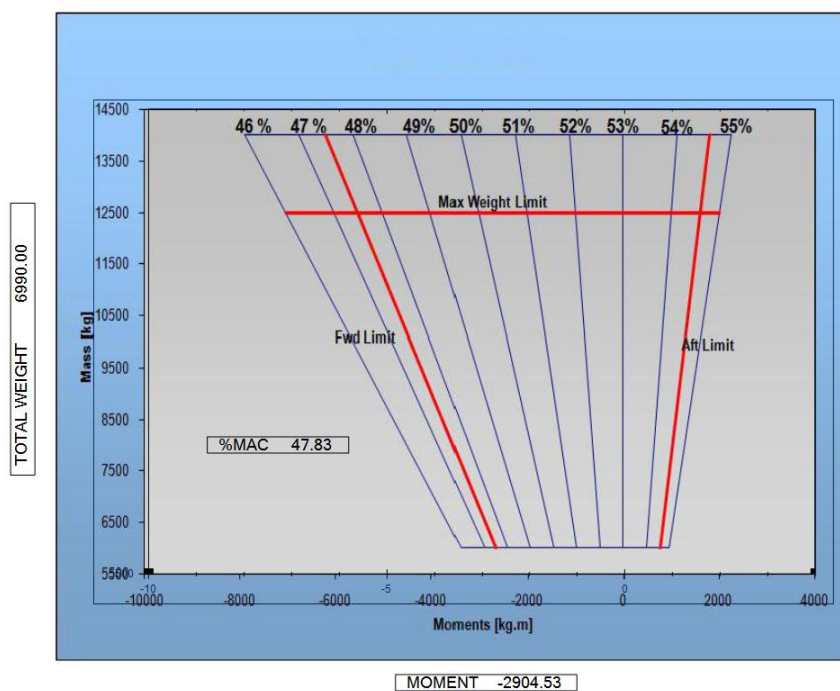
Figure 5: Determination of Aircraft centre-of-gravity.
