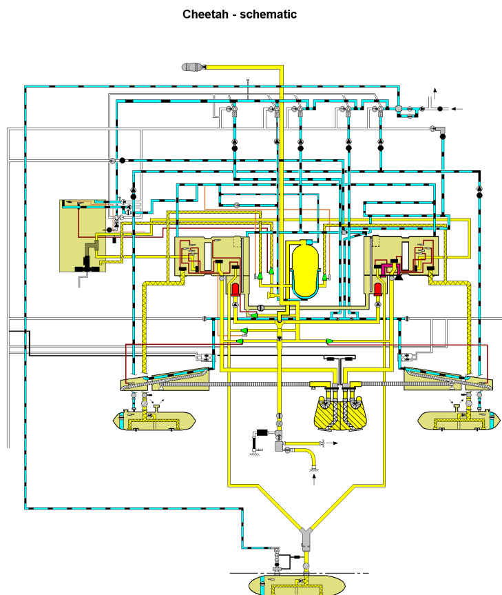
Figure 2: A schematic of the Cheetah fuel system used.
