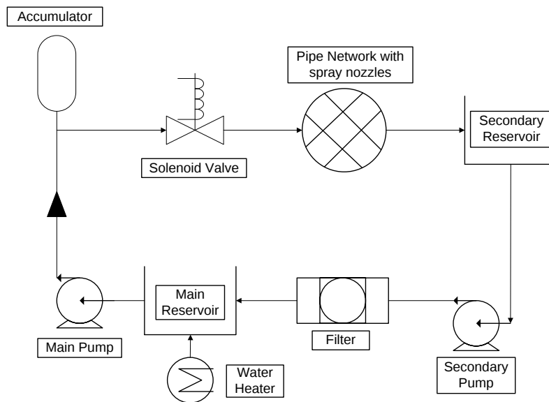
Figure 2: The layout of the washing machine system
