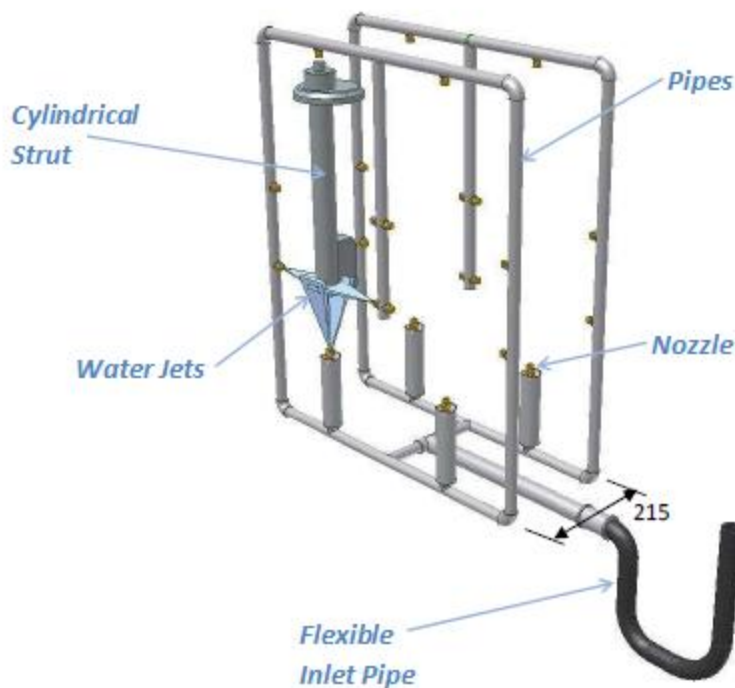
Figure 1: The pipe network of the new washing machine.
