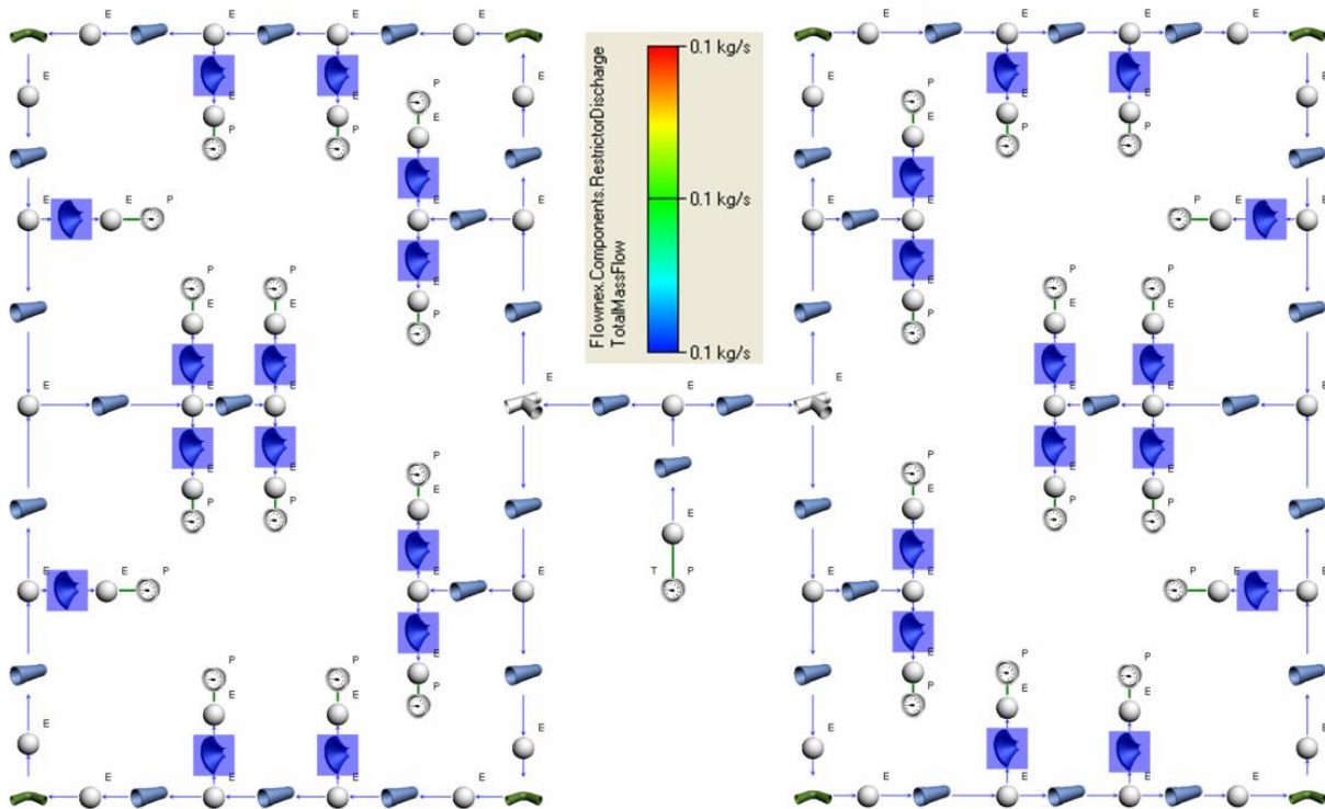
Figure 3: The Flownex® model used for analysis.
