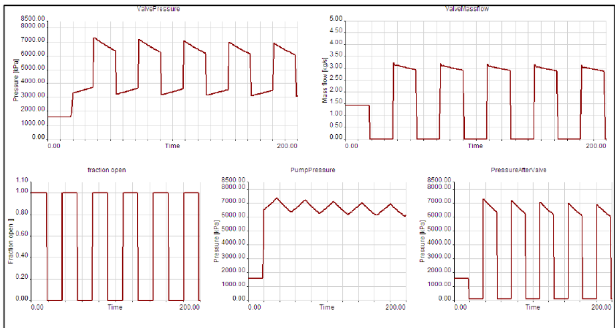
Figure 4: Graphs displaying results of the system simulation.
