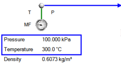
Figure 1: Flownex® Model using a Basic Natural Draft Exhaust Stack Compound Component.
