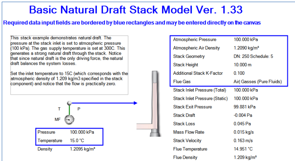
Figure 5: Basic Exhaust Stack Component with Atmospheric Pressure and Temperature at the Entry.
