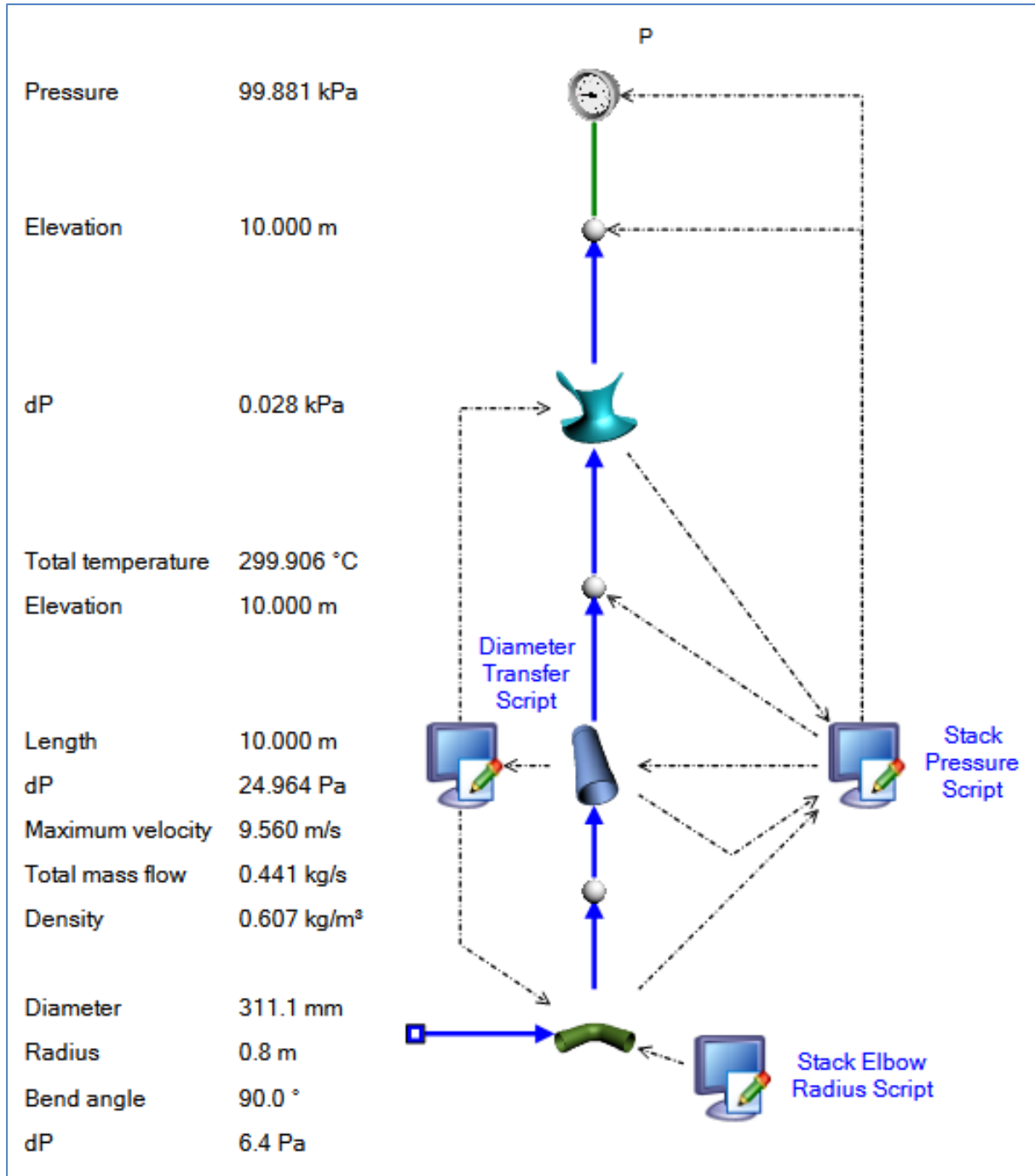
Figure 4: Basic Natural Draft Exhaust Stack Compound Component Inner Elements.
