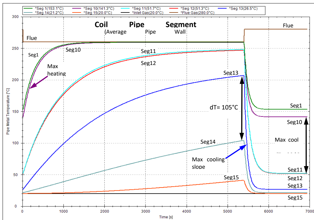
Figure 4: Results of the first cycle in duty mode. The graph is produced using Flownex®.
