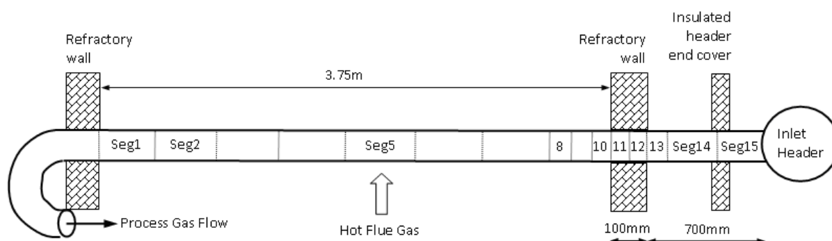
Figure 2: The segment approach to develop the Flownex® model.
