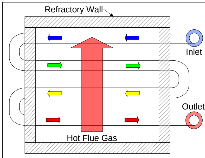
Figure 1: Simplified layout of the fired heater.
