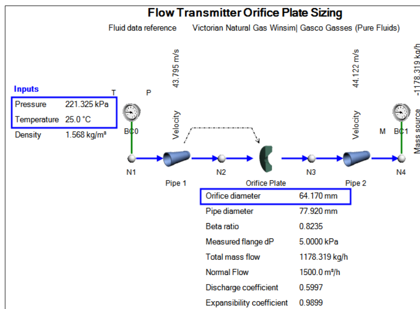
Figure 1: Example Flownex Orifice Plate Pipe Network.
