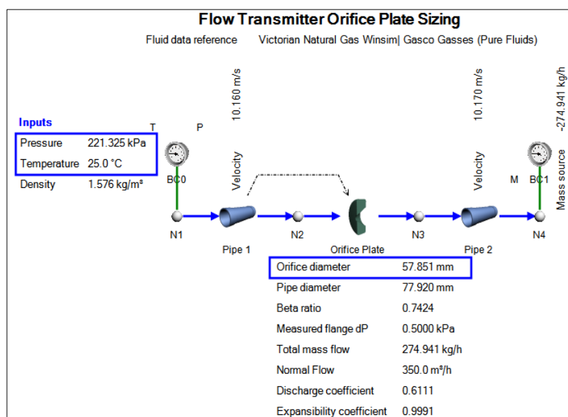
Figure 6: Sizing the Orifice for the Minimum Flow Case (0.5 kPa measured).
