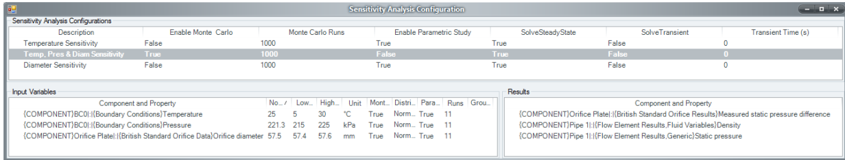
Figure 10: Monte Carlo Analysis Configuration for Temperature, Pressure and Orifice Diameter.
