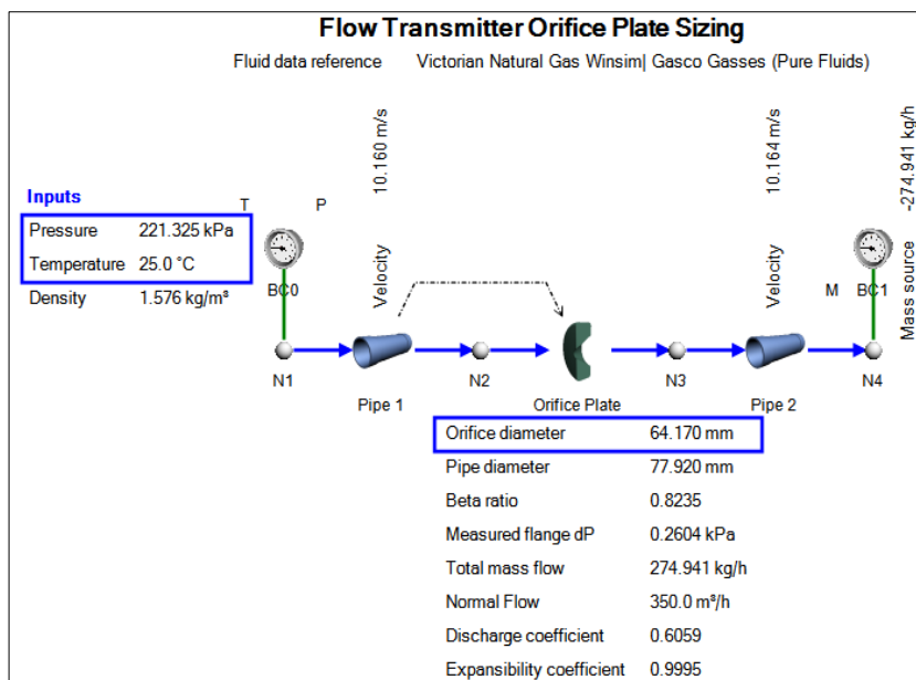
Figure 5: Testing the Low Flow Case (0.3 kPa measured).
