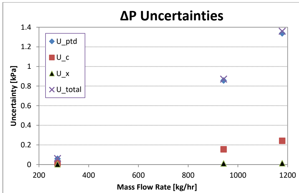
Figure 12: Comparative Pressure Drop Uncertainties as a Function of Flow Rate.
