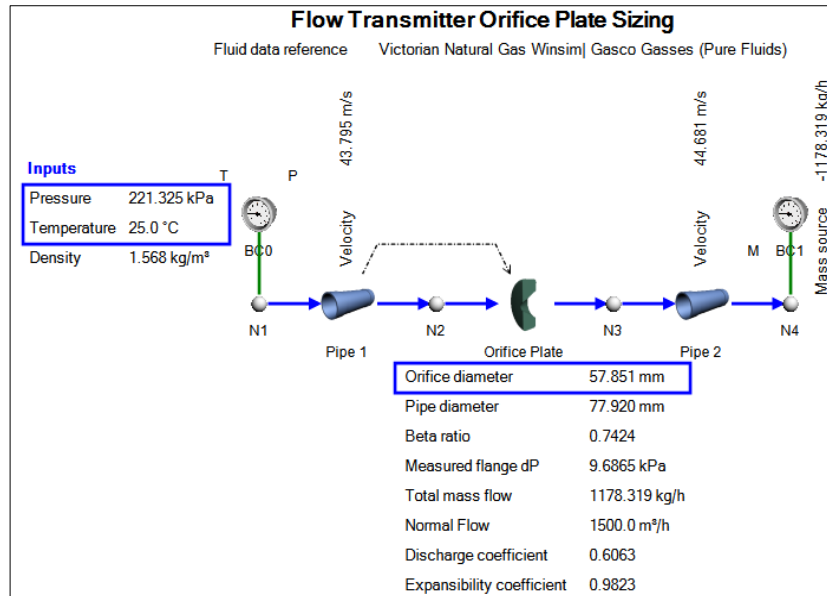
Figure 7: Testing the Orifice for the Maximum Flow Case (9.7 kPa measured).
