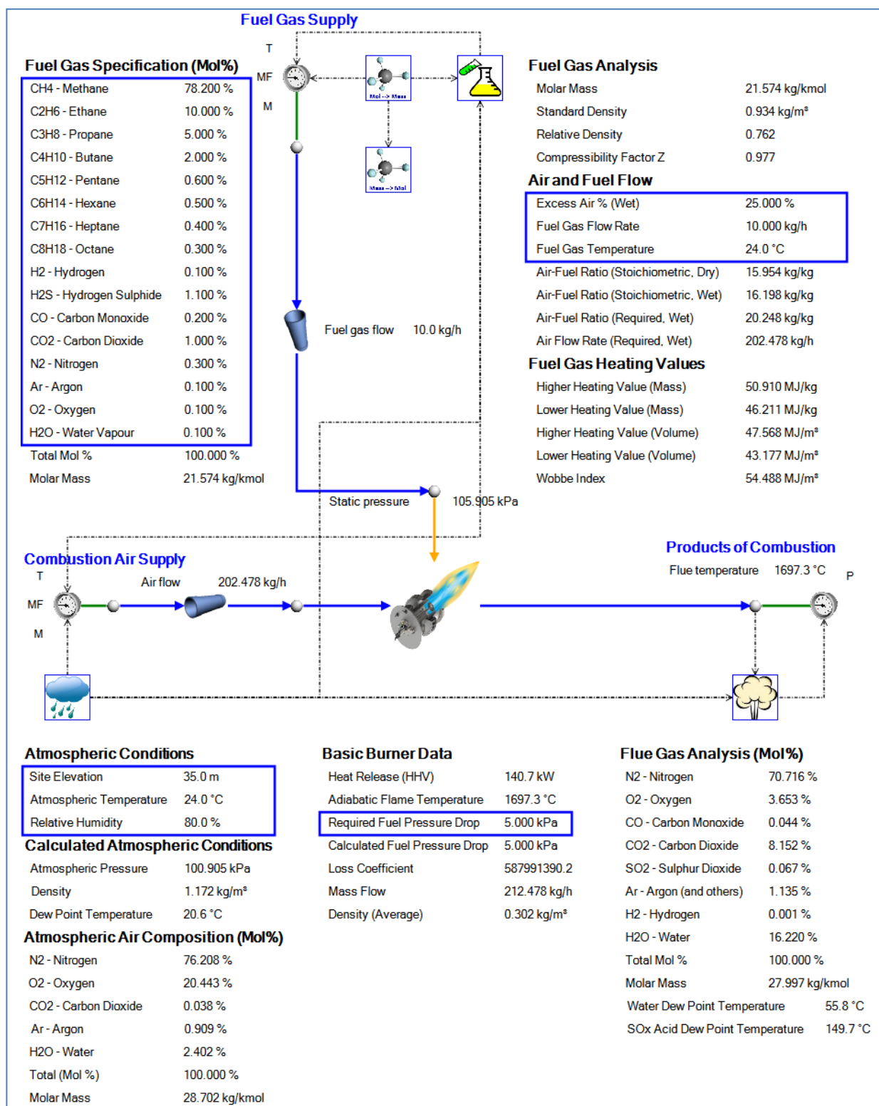
Figure 1: Flownex® Model.
