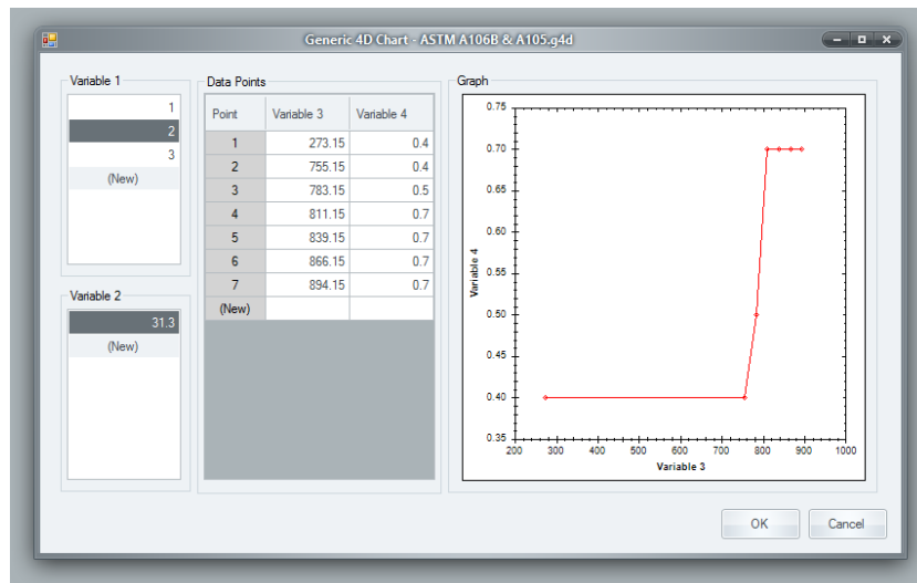
Figure 5: ASME B31.3 Y-Coefficient from Table 304.1.1
