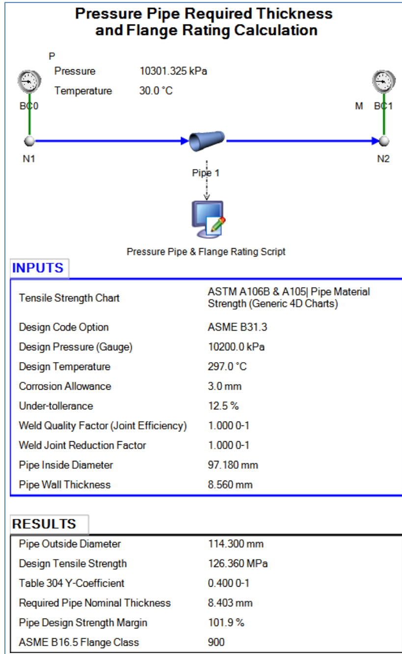
Figure 1: Example Flownex Pressure Pipe Network with Script
