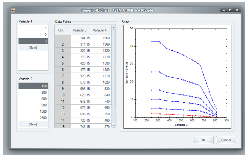
Figure 6: ASME B16.5 Pressure-Temperature Ratings for ASTM A105 Flanges
