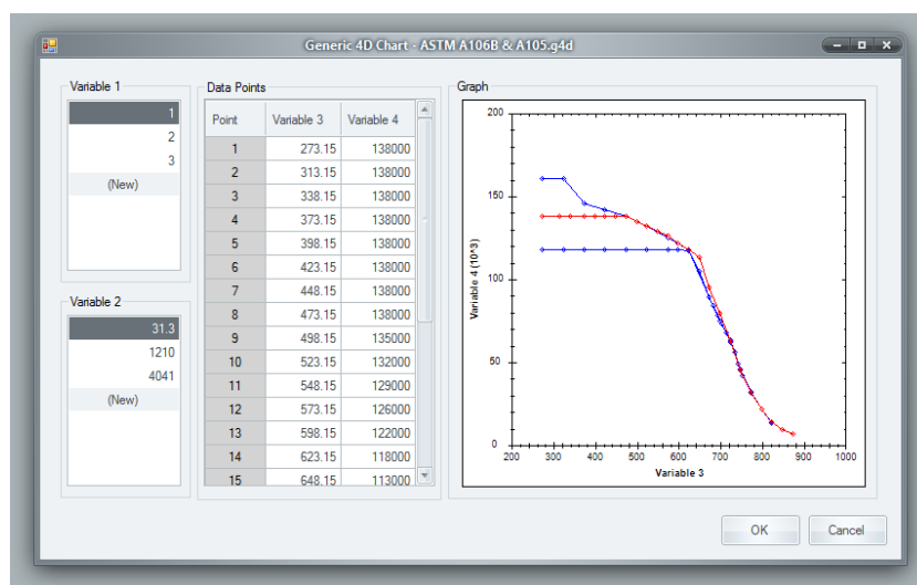
Figure 4: Piping Design Tensile Strength Table for ASME B31.3 Calculations for ASTM A106 Gr B Material
