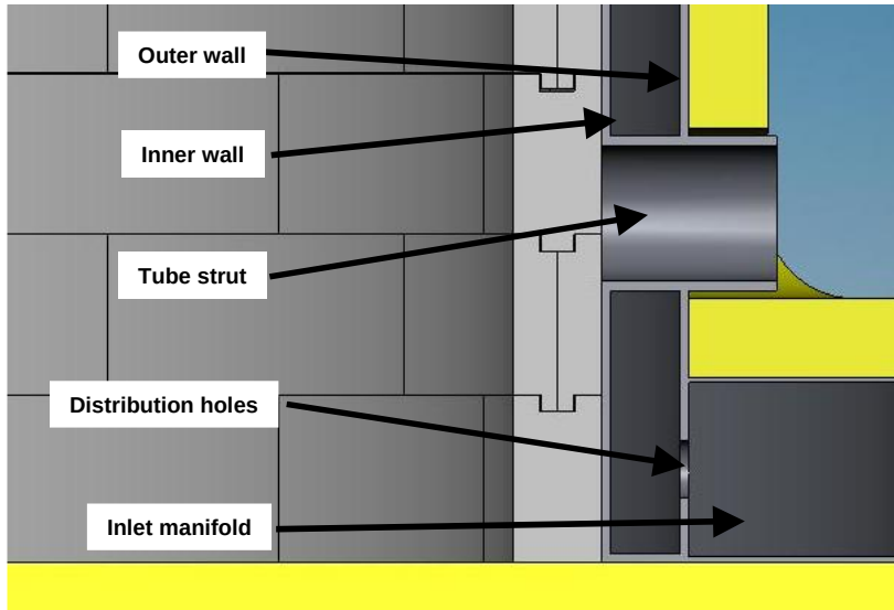
Figure 2: Detail of the inlet manifold and water distribution holes around the circumference.
