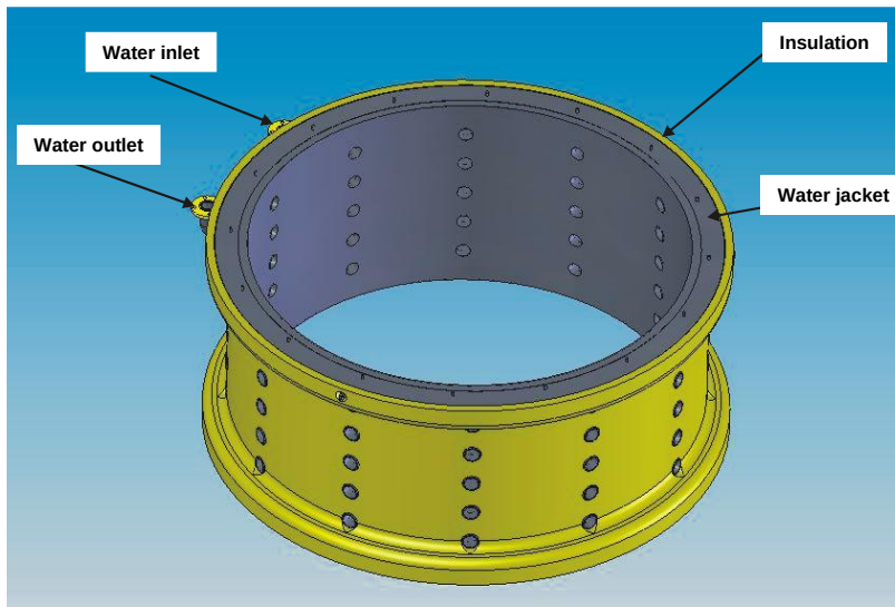
Figure 1: Solid model of the water jacket layout.
