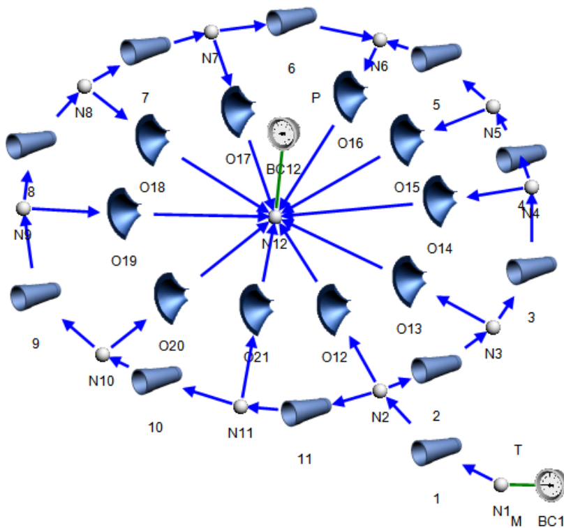
Figure 3: Flownex network of the water jacket inlet manifold and distribution holes.
