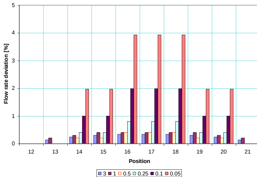
Figure 4: Simulated deviation in flow rate at the different openings for various different total flow rates.
